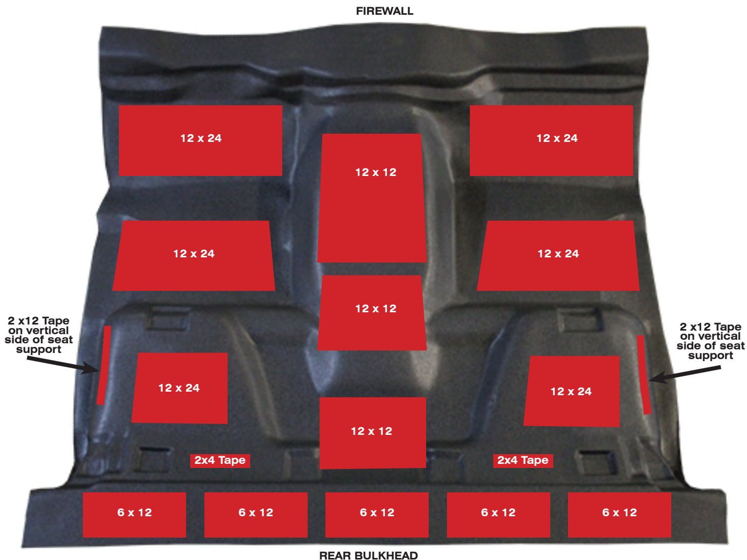
FIG. 2 Install damping material in these approximate locations. The perfect placement is not critical. But good adhesion is key. Make sure to press material in place with roller to ensure good adhesion. (View from above)
