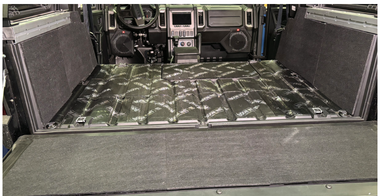
TAILGATE, CARGO SIDEWALLS, & CARGO FLOOR SOUND CONTROL
